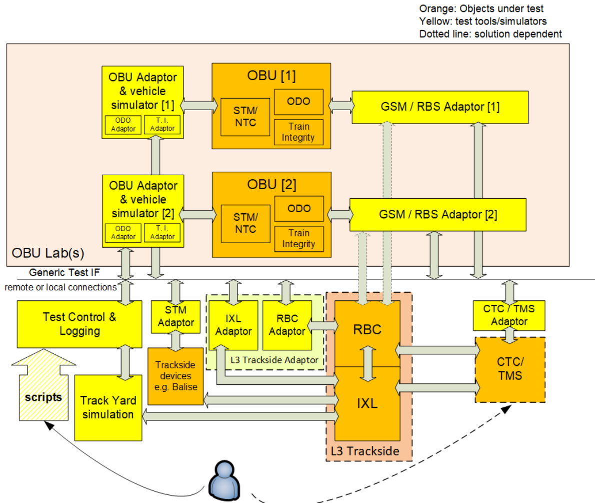
Use case "Environment for validation of Moving Block"
