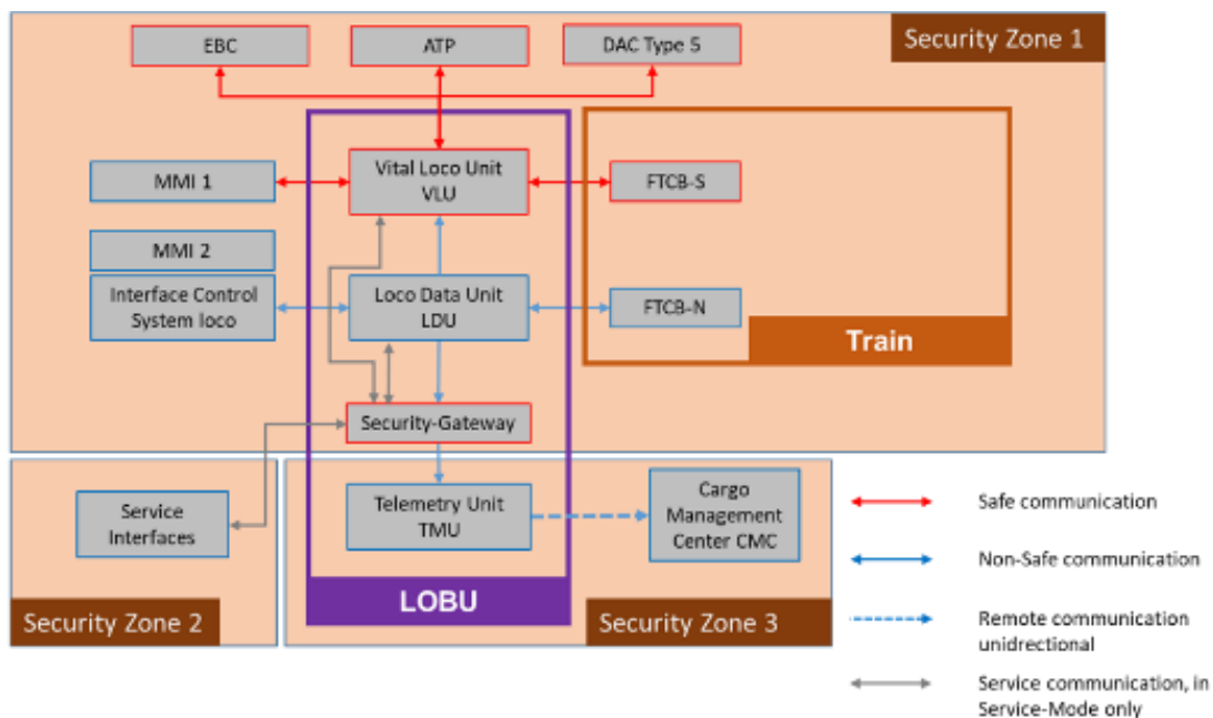
LOBU and architecture
