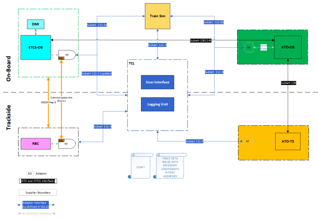
ATO Testing Architecture
