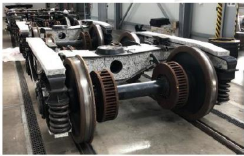
A number of wheelsets solutions have been employed for the noise field tests
